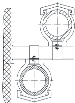
With opposite steel clamp on a steel profile (vertical and hanging construction)
